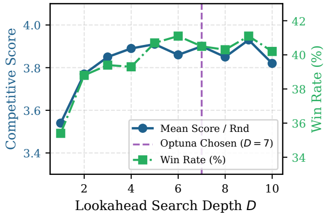
(a) Competitive Combat vs. Lookahead Depth
